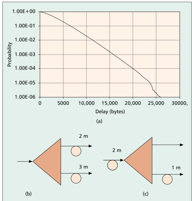
■ Figure 5. a) The probability that a randomly chosen byte is experiencing a delay greater than the given value in an output-buffered switch, for self-similar traffic, with a mean traffic level of 80 percent; b and c) an example of sharing delay lines. The subsystem in b) requires 5 m of fiber delay line, whereas only 3 m are required in c), because the smallest delay line has been moved in front of the splitter.
